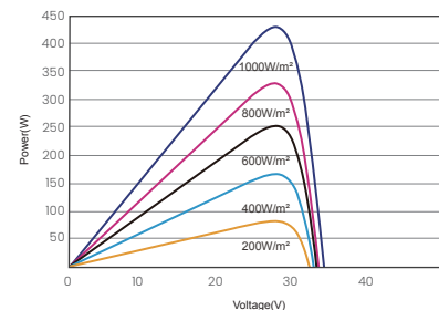
P-V CURVES OF PV MODULE(430W)
